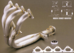
① EXHAUST MANIFOLD KIT
